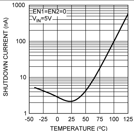
Figure 5. AVIN Shutdown Current vs Temperature
