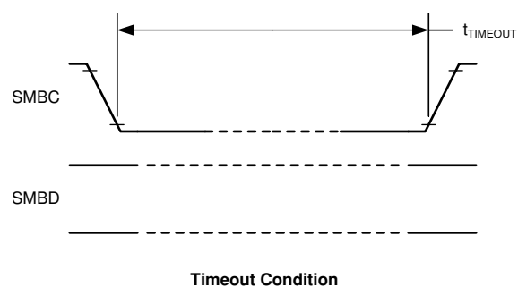
Figure 7-1. SMBus Timing Diagram
