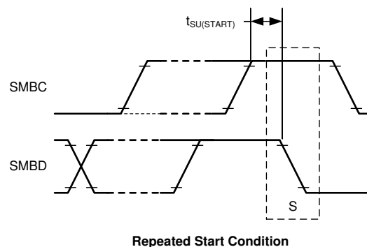
Figure 7-1. SMBus Timing Diagram
