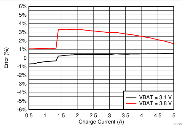
VBUS = 9 V Figure 7-4. Charge Current Accuracy vs Charge Current I²C Setting
