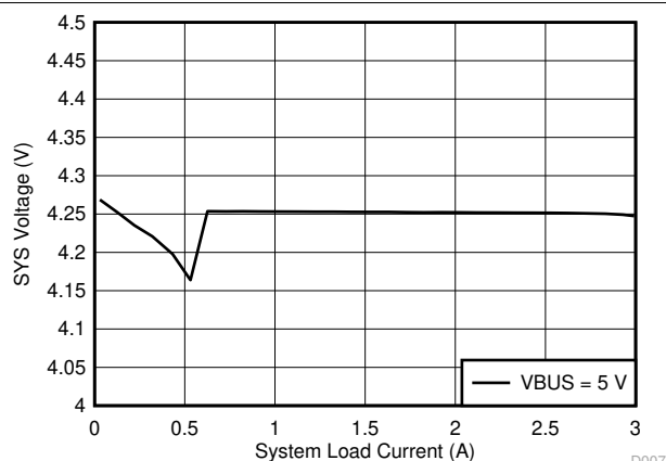
VBAT = 4.2 V Figure 7-6. SYS Voltage Regulation vs System Load Current
