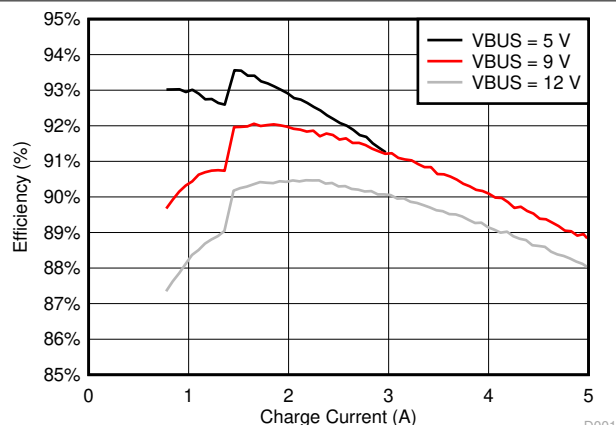
VBAT = 3.8 V DCR = 10 mΩ Figure 7-1. Charge Efficiency vs Charge Current
