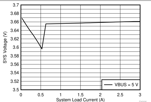
VBAT = 2.9 V VBUS = 5 V SYSMIN = 3.5 V Figure 7-5. SYS Voltage Regulation vs System Load Current
