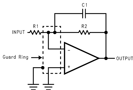
Figure 58. Inverting Amplifier
