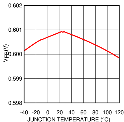
Figure 6-5. V_{FB} vs Temperature
