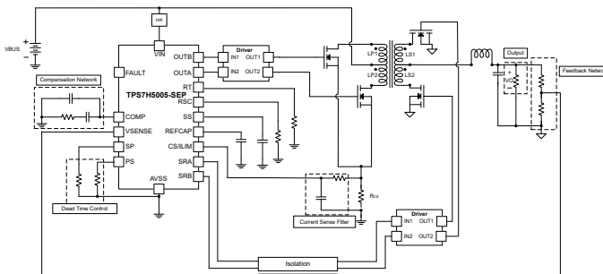
Typical Application for TPS7H5005-SEP
