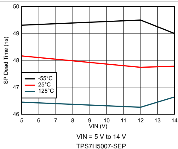
Figure 7-56. SP Dead Time Variation
