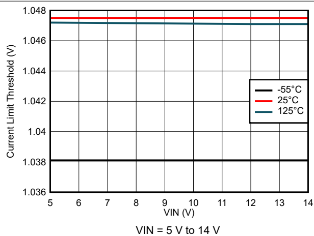
Figure 7-18. Current Limit Threshold Variation
