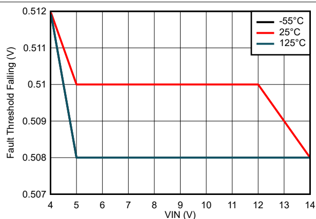
Figure 7-32. FAULT Threshold Falling Variation
