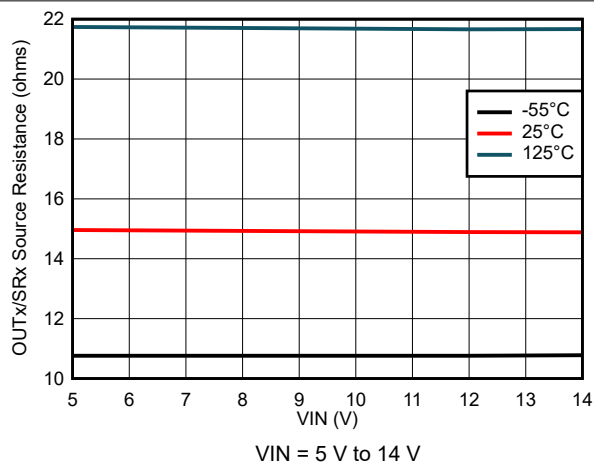
Figure 7-62. Output Source Resistance Variation
