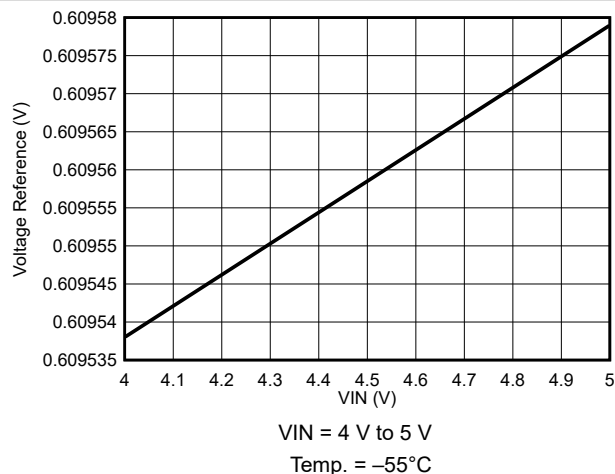
Figure 7-11. Voltage Reference Variation
