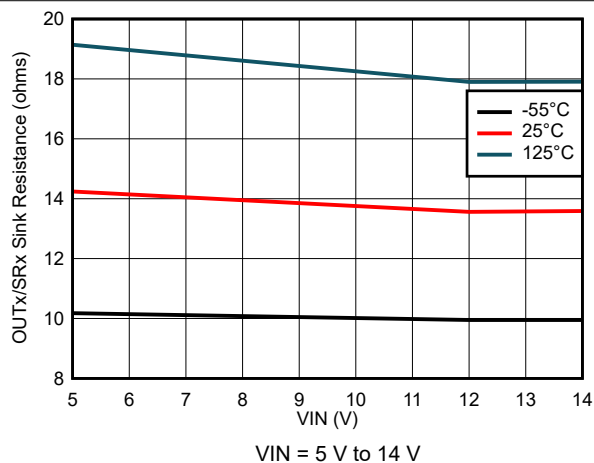
Figure 7-64. Output Sink Resistance Variation
