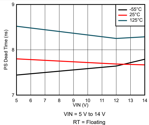
Figure 7-42. PS Dead Time Variation
