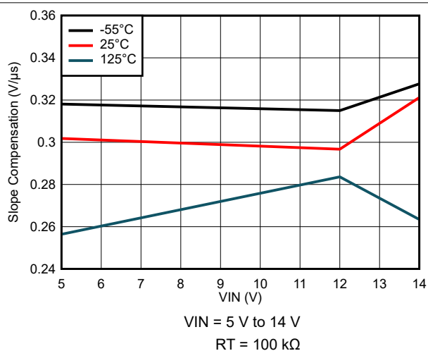
Figure 7-70. Slope Compensation Variation
