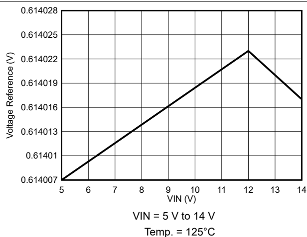
Figure 7-16. Voltage Reference Variation
