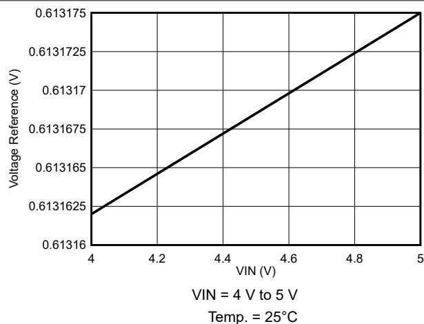
Figure 7-13. Voltage Reference Variation
