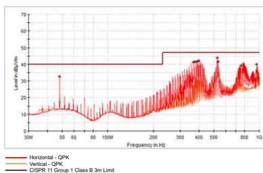
Figure 9-136. TPSM82823 Radiated Emissions
