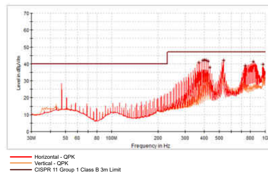
Figure 9-84. TPSM82822 Radiated Emissions
