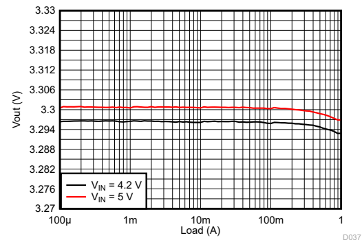
Figure 9-44. Load Regulation
