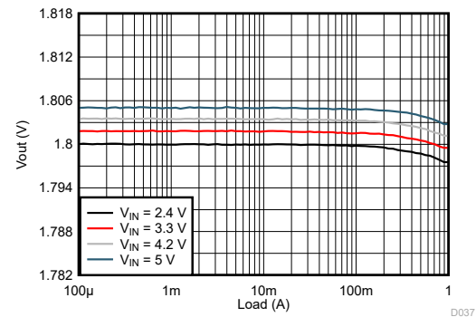
Figure 9-42. Load Regulation
