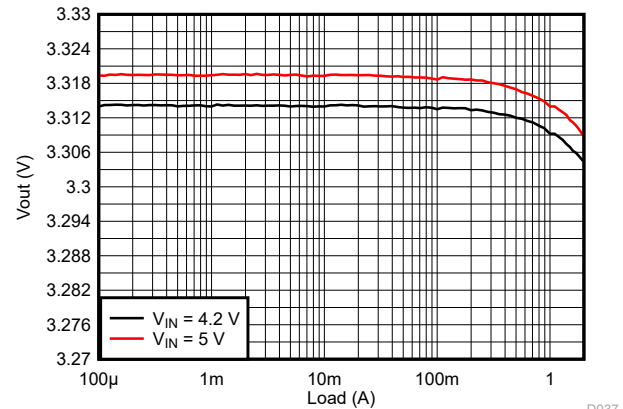
Figure 9-101. Load Regulation
