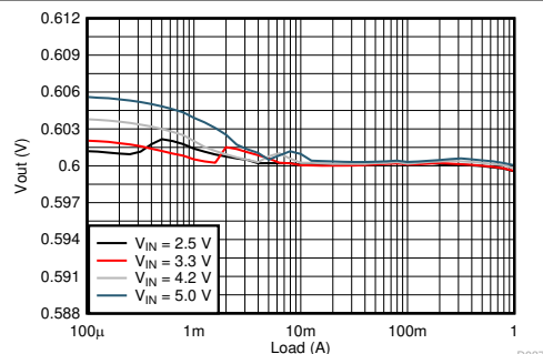
Figure 9-16. Load Regulation
