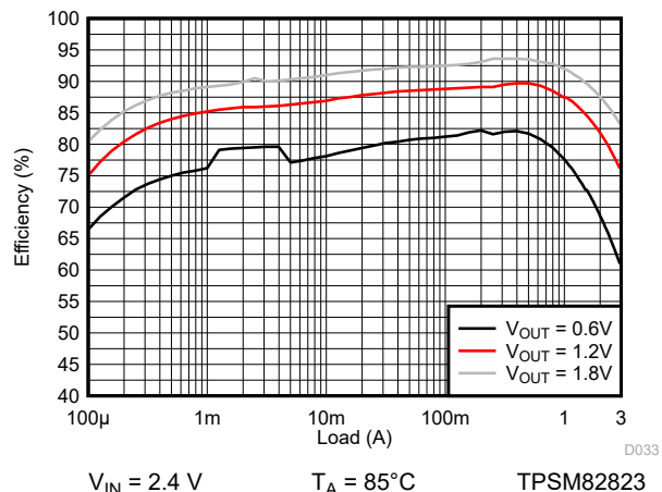
Figure 9-117. Efficiency
