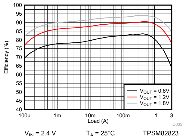
Figure 9-116. Efficiency
