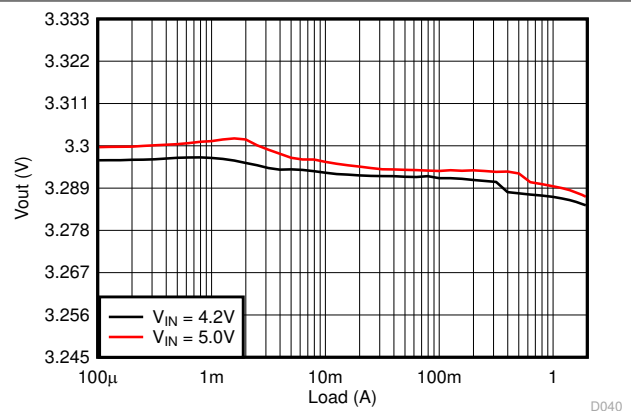
Figure 9-68. Load Regulation
