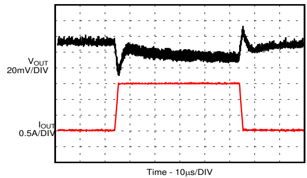
Figure 9-80. Load Transient
