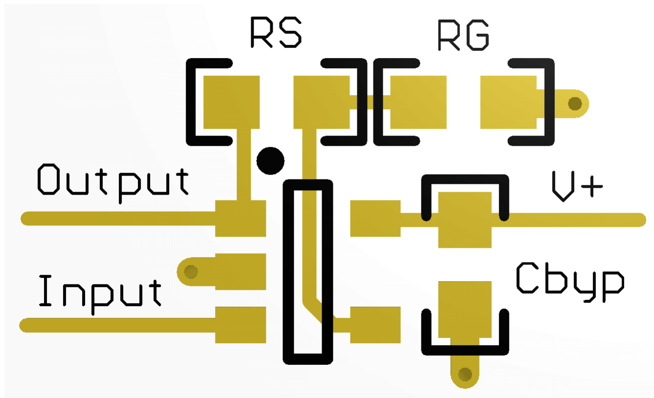
Figure 55. Layout Recommendation
