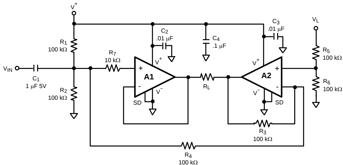
Figure 53. Bridge Amplifier
