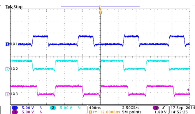
Figure 49. 180° Out of Phase
