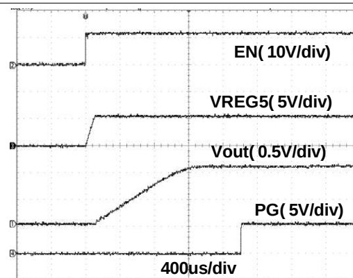
Figure 12. Start-Up Waveform
