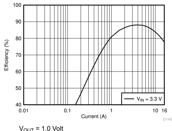
Figure 8-2. Efficiency in Forced-PWM-Four-Phase Mode
