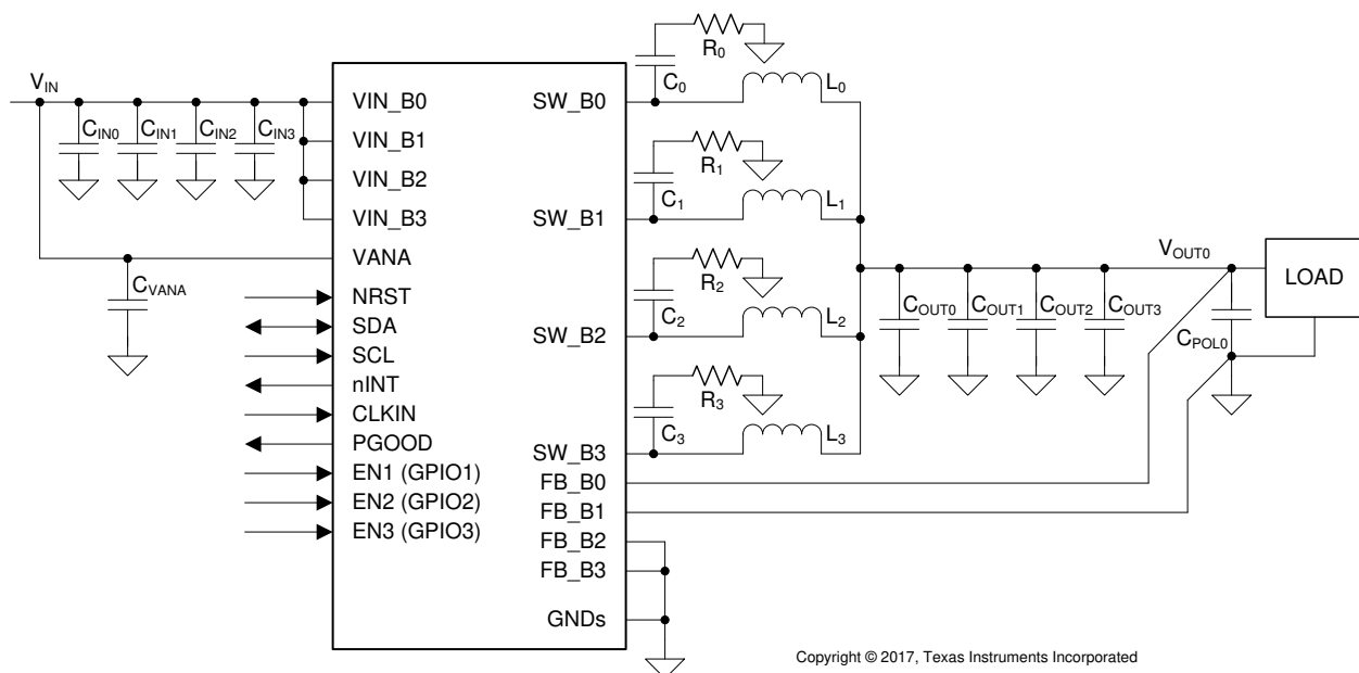
Figure 8-1. 4-Phase Configuration
