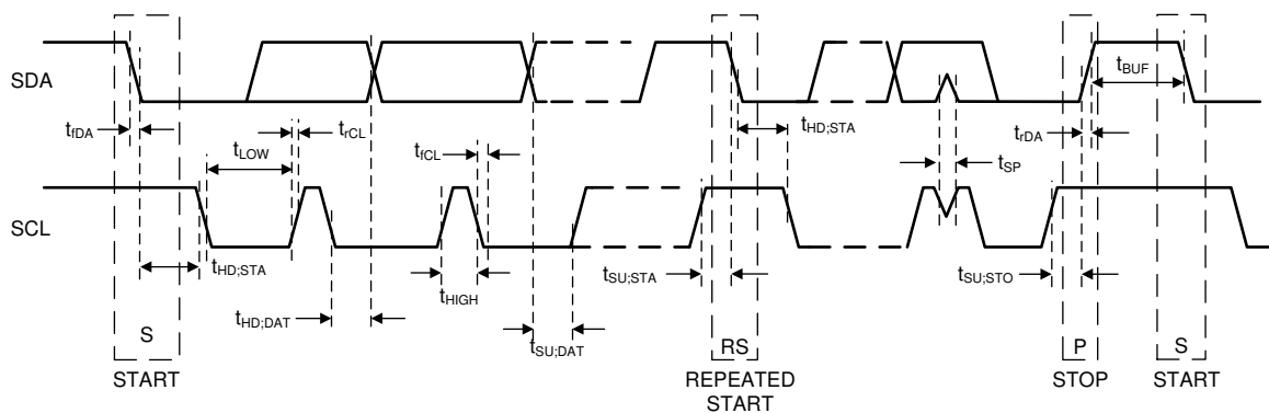
Figure 6-1. I²C Timing
