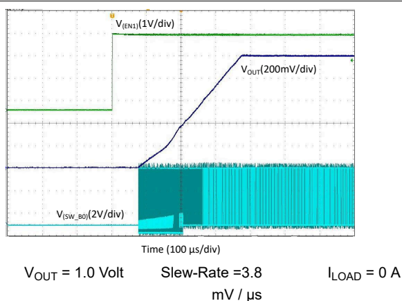
Figure 8-6. Start-Up With EN1, Forced-PWM-Four-Phase Mode
