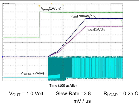
Figure 8-7. Start-Up With EN1, Forced-PWM-Four-Phase Mode
