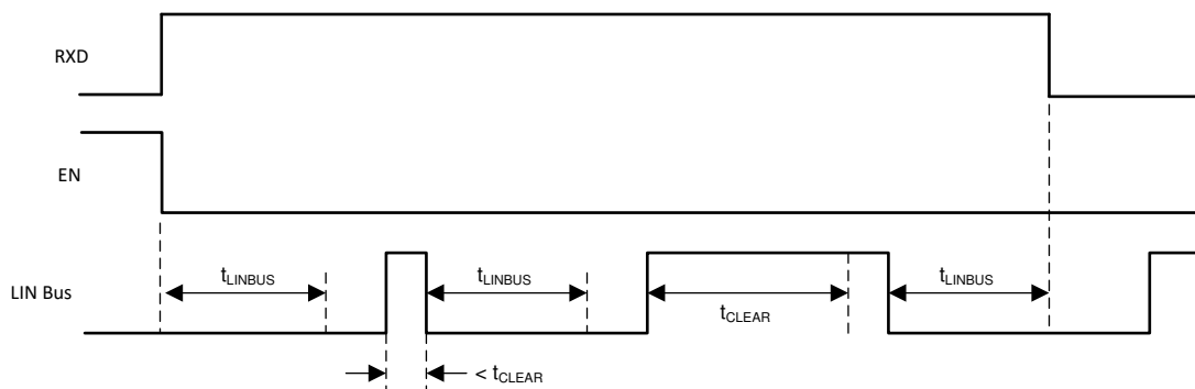
Figure 9-3. Bus Fault: Entering Sleep Mode with Bus Stuck Dominant Fault, Clearing, and Wakeup
