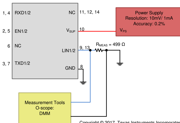
Figure 8-6. Test Circuit for I_{BUS\_PAS\_dom} ; TXD = Recessive State V_{BUS} = 0 V, Parameter 13
