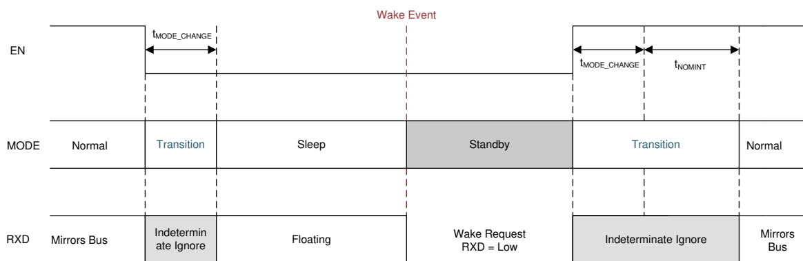
Figure 8-14. Mode Transitions
