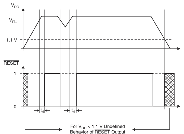
Figure 7-1. Timing Diagram
