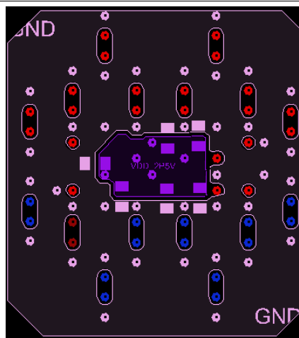
Figure 32. Bottom Layer
