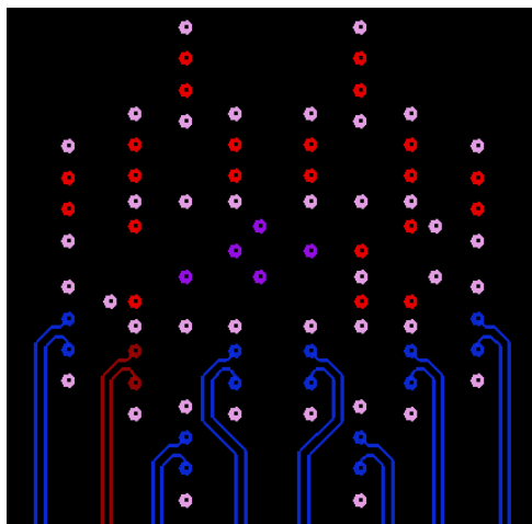
Figure 30. Internal Signal Layer 1
