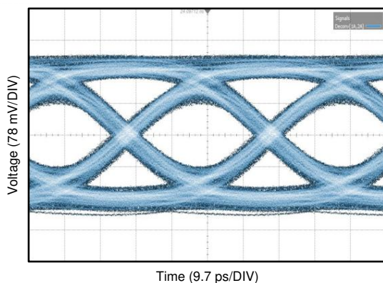
Figure 27. 25.78125 Gbps Limiting Mode with FIR
