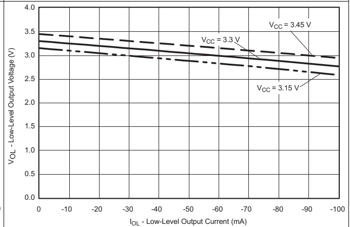
Figure 5. Low-Level Output Voltage vs Low-Level Output Current, V_{OL} vs I_{OL}
