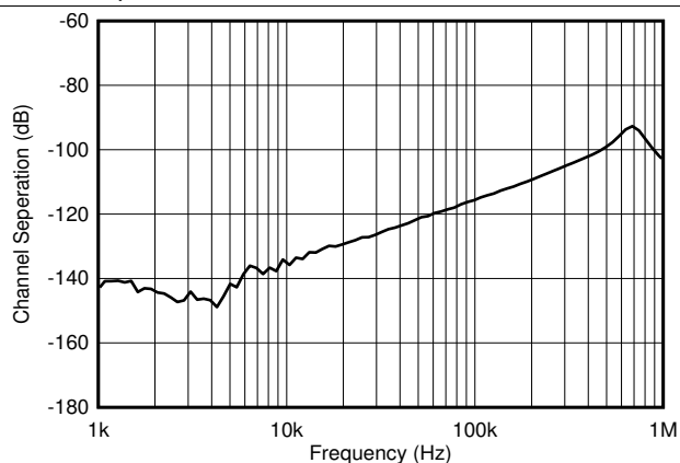
Figure 38. Channel Separation
