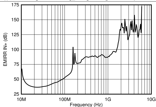
Figure 37. EMIRR vs Frequency
