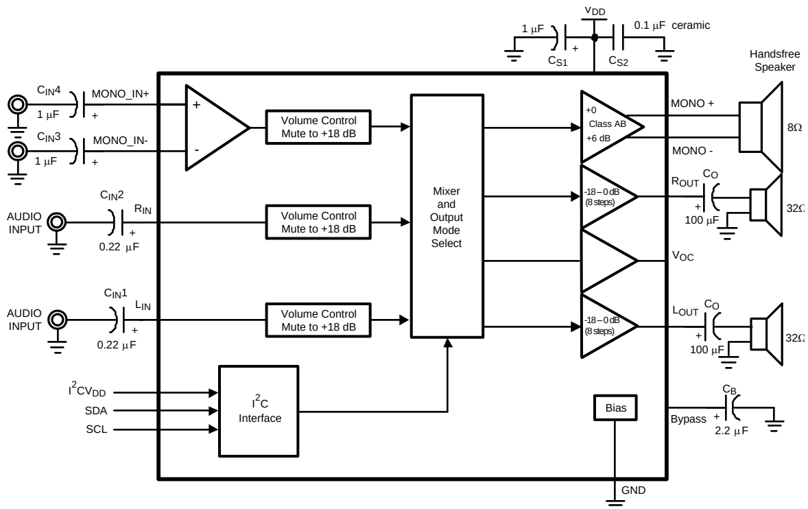
Figure 2. Single-Ended Configuration
