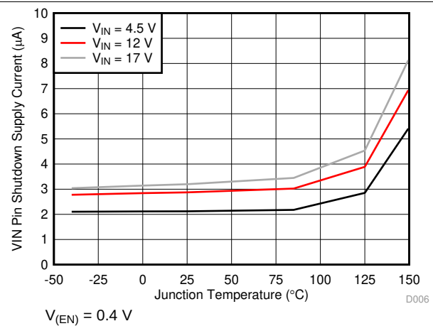
Figure 5. VIN Pin Shutdown Current vs Junction Temperature
