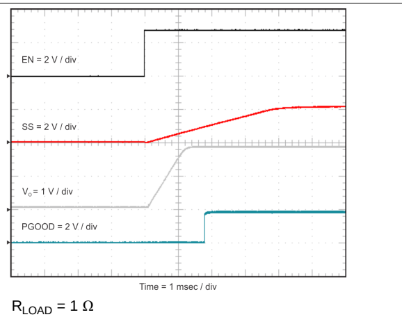
Figure 44. EN Startup
