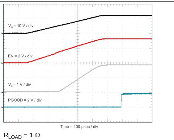
Figure 43. V_{IN} Startup
