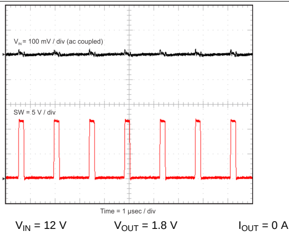
Figure 41. Input Voltage Ripple, No Load
