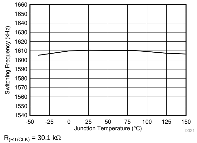
Figure 20. Switching Frequency vs Junction Temperature (1600 kHz)
