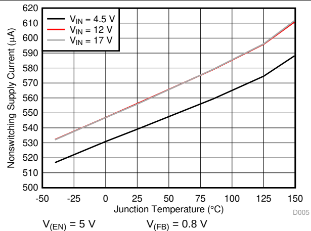
Figure 4. VIN Pin Nonswitching Supply Current vs Junction Temperature
