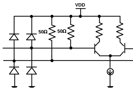
Figure 12. Equivalent Input Structure
