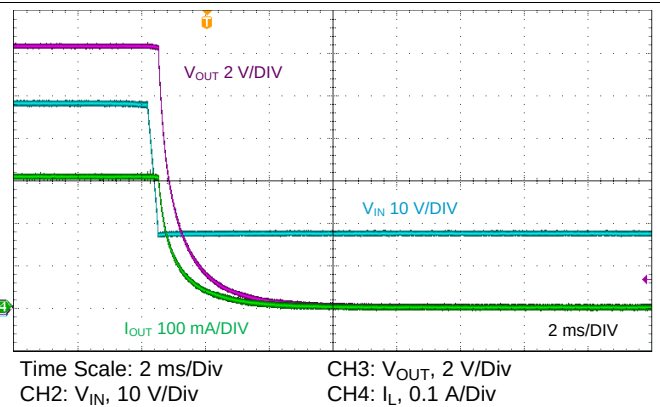
Figure 88. Shutdown Waveforms
