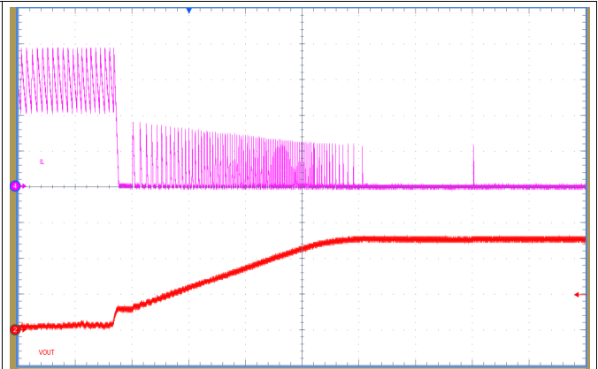
Figure 62. Short-Circuit Recovery
