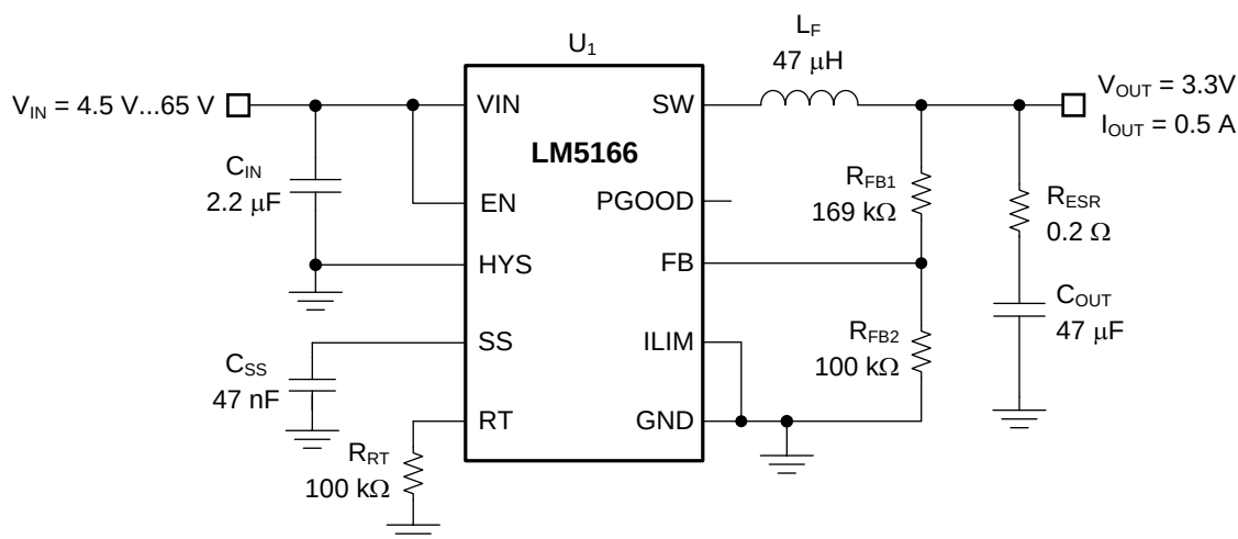
Figure 63. Schematic for Design 2 With V_{IN(nom)} = 12 V, V_{OUT} = 3.3 V, I_{OUT(max)} = 500 mA, F_{SW(nom)} = 200 kHz
