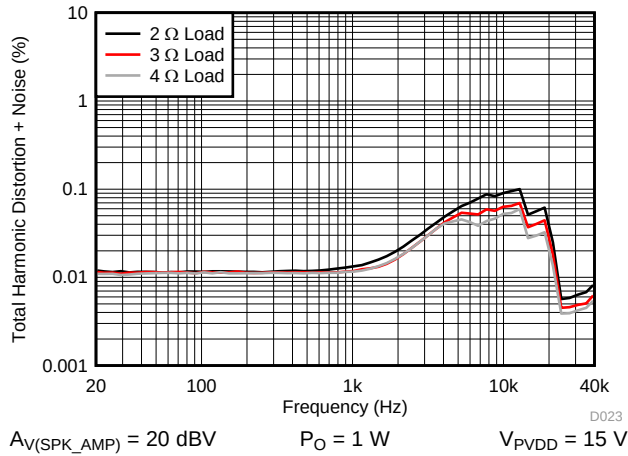
Figure 49. THD+N vs Frequency – PBTl
