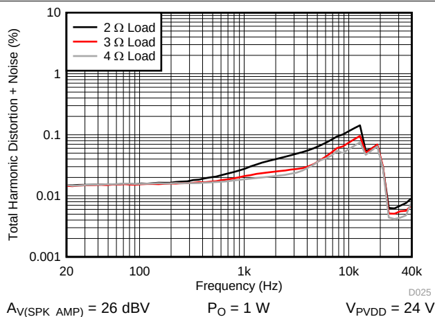
Figure 51. THD+N vs Frequency – PBTl
