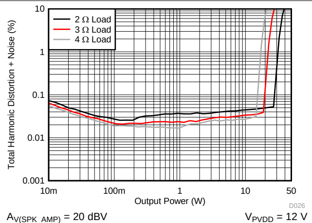
Figure 52. THD+N vs Power – PBTl
