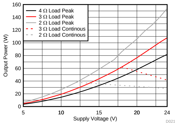
Figure 47. Output Power vs PVDD – PBTl
