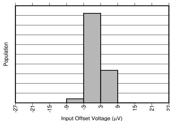
Figure 6-4. INA310A4 Input Offset Production Distribution
