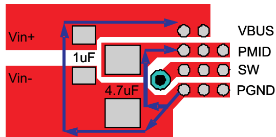
Figure 39. Input Capacitor Position and PCB Layout Example
