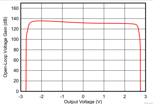
Figure 6-5. Open-Loop Gain vs Output Voltage
