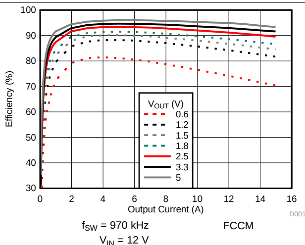
Figure 4. Efficiency vs. Output Current
