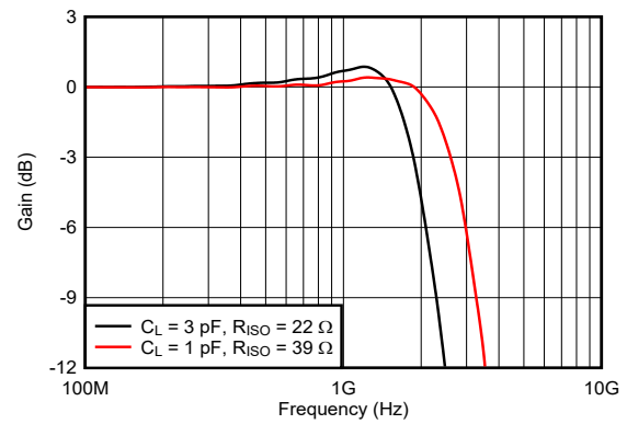
Figure 6-8. Frequency Response vs Cap Load with Recommended R_{ISO}
