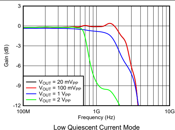
Figure 6-2. Frequency Response vs Output Voltage
