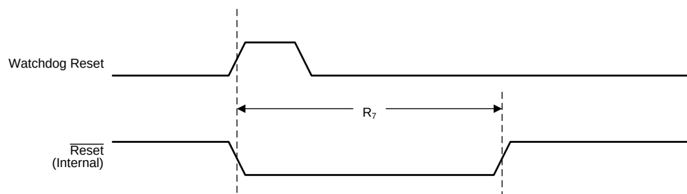
Figure 5-11. Watchdog Reset Timing
