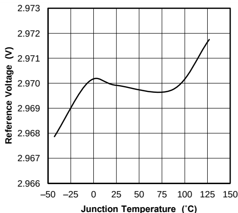
Figure 7. VREF Voltage
