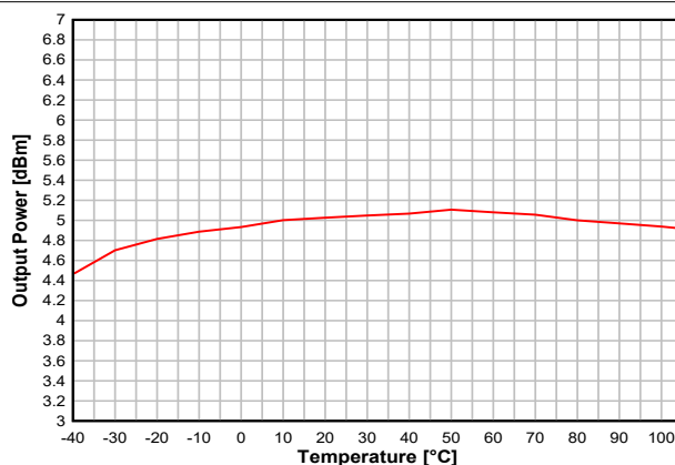
Figure 7-22. Output Power vs. Temperature (BLE 1Mbps, 2.44GHz, +5dBm)
