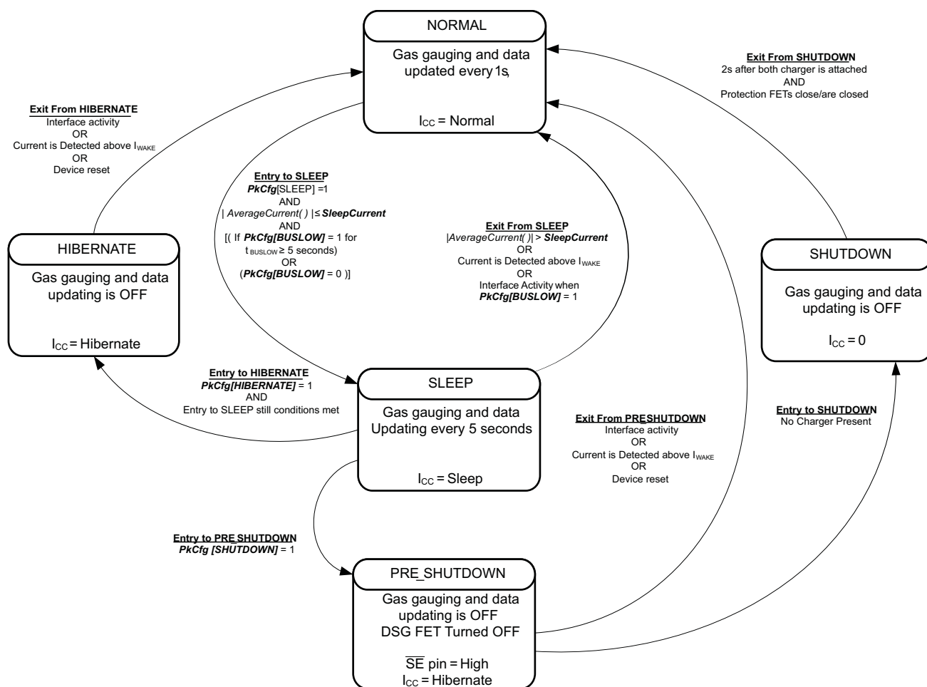
Figure 5-1. Power Mode Diagram
