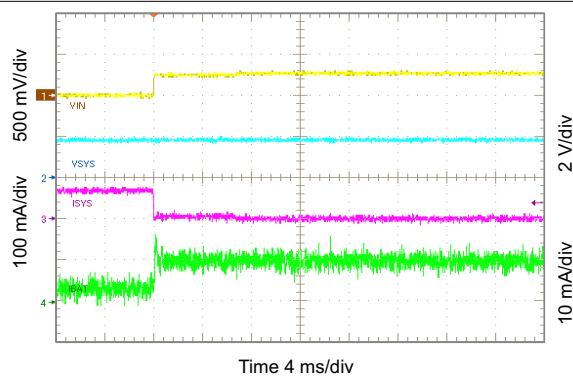
Figure 10-5. Exiting DPPM Mode
