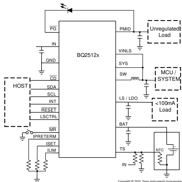
Simplified Schematic
