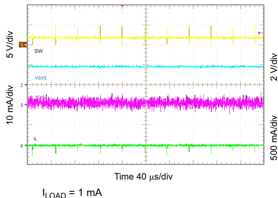
Figure 10-28. Light Load Operation Showing SW
