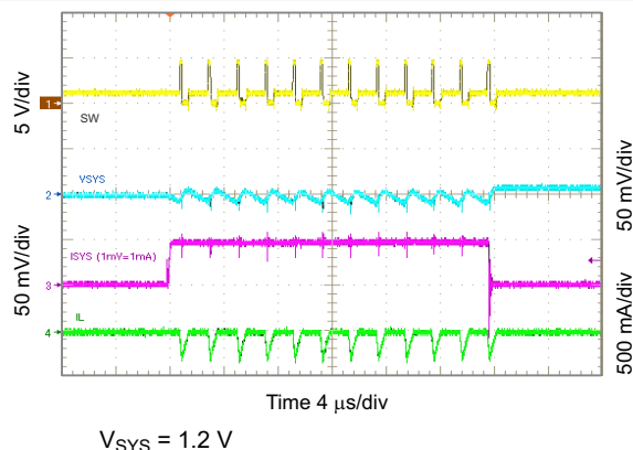
Figure 10-33. 1.2 V_{SYS} Load Transient, 0 to 50 mA
