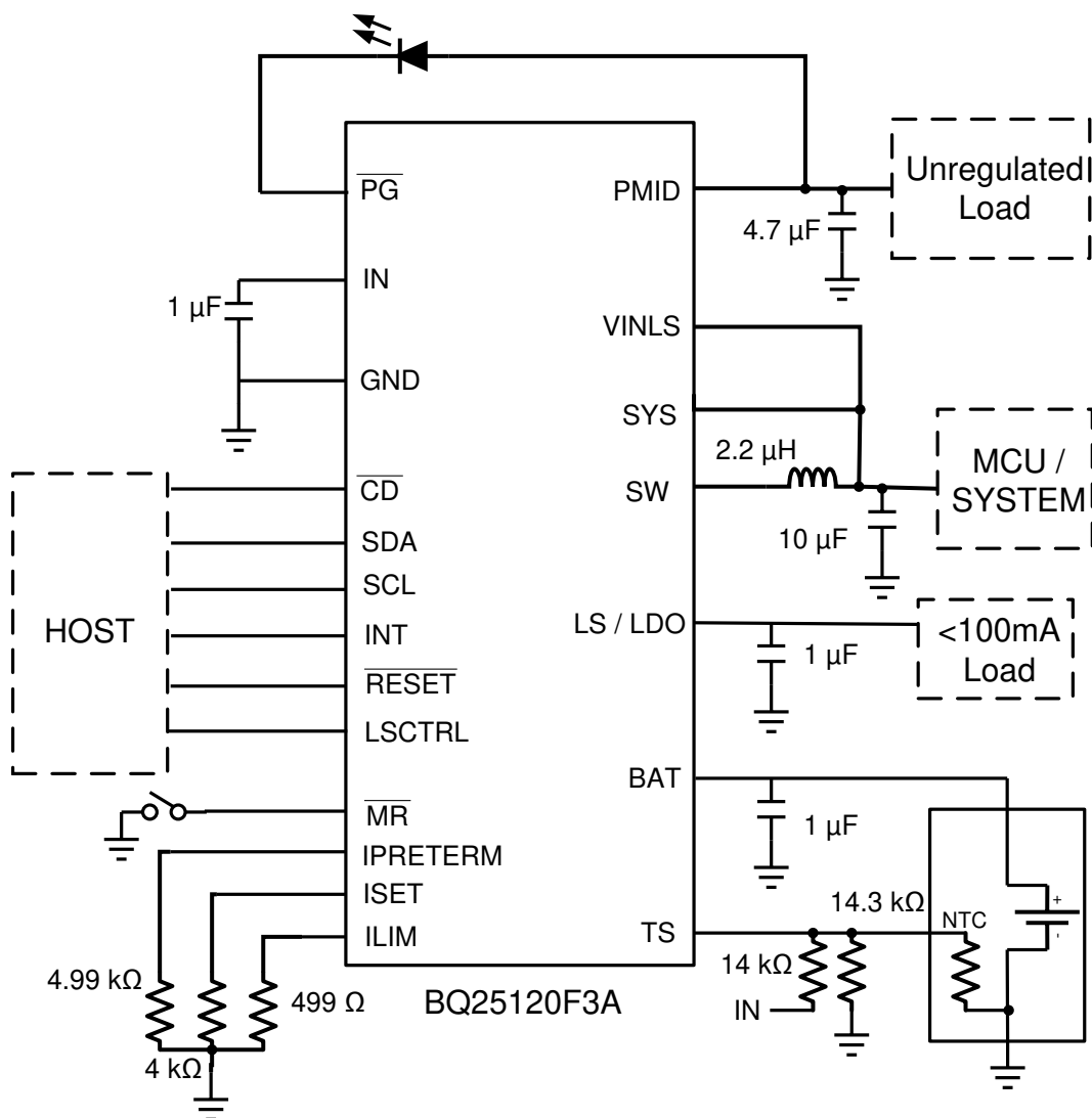
Figure 10-1. Typical Application Circuit
