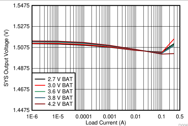
T_A = 25^\circ\text{C} V_{\text{SYS}} = 1.5\text{ V} Figure 10-16. 1.5 V_{\text{SYS}} Load Regulation
