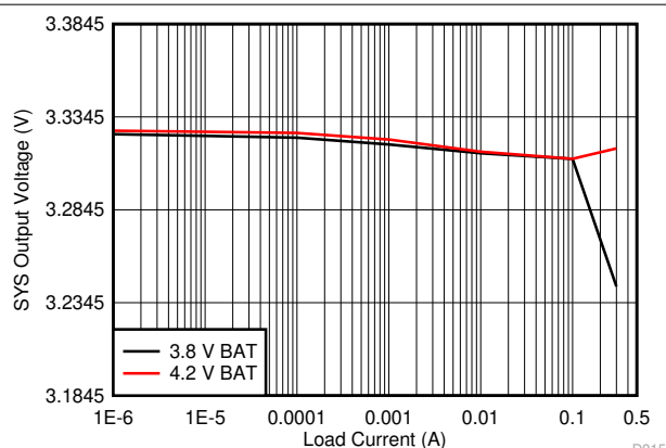
T_A = 25^\circ\text{C} V_{\text{SYS}} = 3.3\text{ V} Figure 10-19. 3.3 V_{\text{SYS}} Load Regulation
