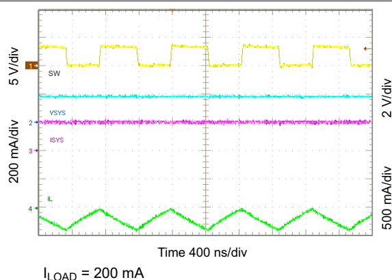
Figure 10-31. Light Load Operation Showing SW
