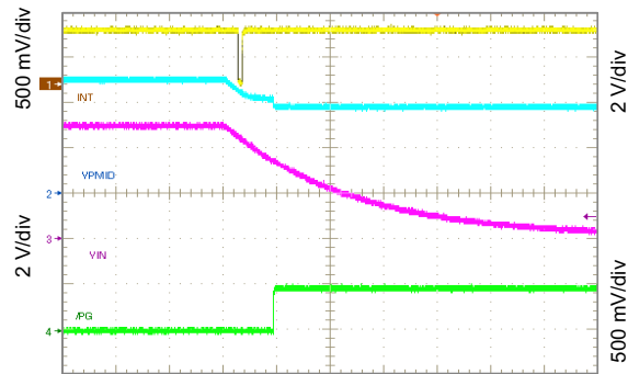
Time 2 ms/div Figure 10-60. Show \overline{\text{PG}} and \overline{\text{INT}} Timing ( \text{V}_{\text{IN}} Removal)
