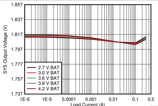
T_A = 25^\circ\text{C} V_{\text{SYS}} = 1.8\text{ V} Figure 10-17. 1.8 V_{\text{SYS}} Load Regulation
