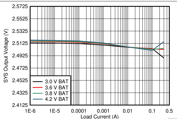
T_A = 25^\circ\text{C} V_{\text{SYS}} = 2.5\text{ V} Figure 10-18. 2.5 V_{\text{SYS}} Load Regulation
