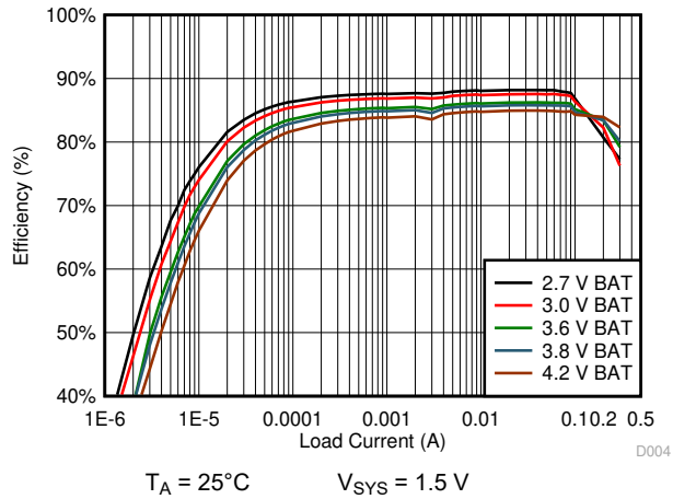
Figure 10-11. 1.5 V_{\text{SYS}} System Efficiency
