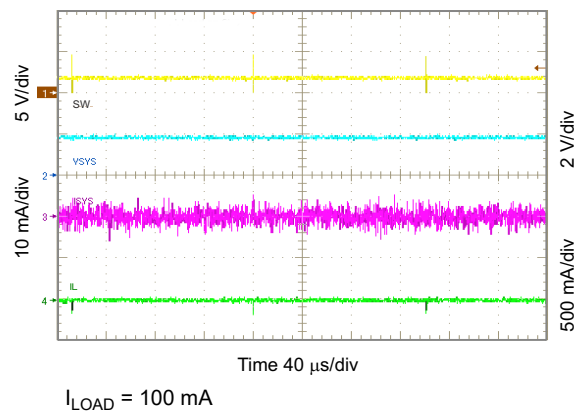
Figure 10-27. Light Load Operation Showing SW
