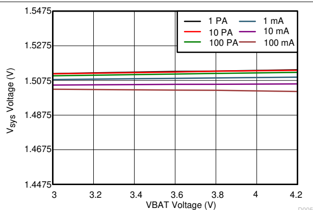
T_A = 25^\circ\text{C} V_{\text{SYS}} = 1.5\text{ V} Figure 10-21. 1.5 V_{\text{SYS}} Line Regulation
