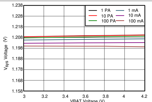
T_A = 25^\circ\text{C} V_{\text{SYS}} = 1.2\text{ V} Figure 10-20. 1.2 V_{\text{SYS}} Line Regulation
