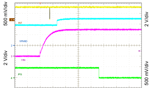
Time 10 ms/div Figure 10-59. Show \overline{\text{PG}} and \overline{\text{INT}} Timing ( \text{V}_{\text{IN}} Insertion)
