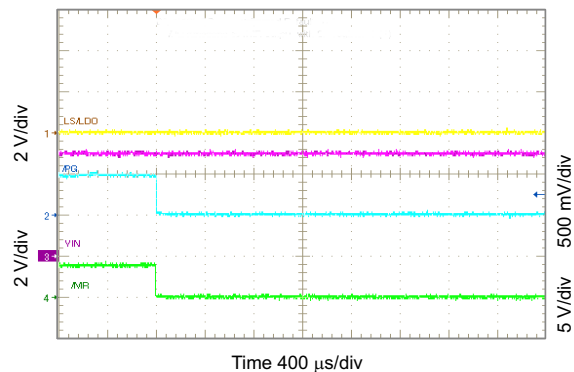
Time 400 μs/div Figure 10-61. \overline{\text{PG}} Functions as Shifted \overline{\text{MR}} Output
