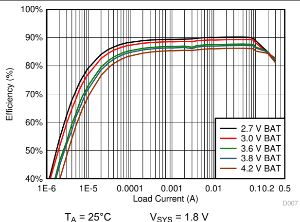
Figure 10-12. 1.8 V_{\text{SYS}} System Efficiency
