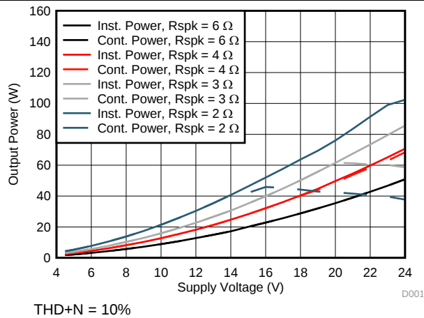
Figure 18. Output Power vs Supply Voltage – PBTL
