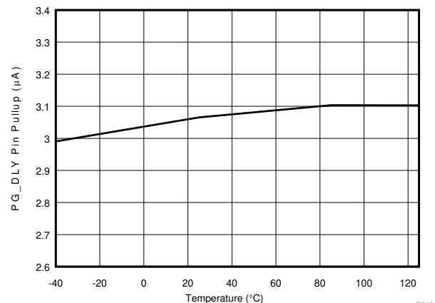
Figure 7-10. PG_DLY Pin Pullup Current vs Temperature, PG_DLY = 0.5 V
