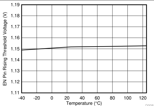
Figure 7-8. EN Pin Threshold Raising vs Temperature
