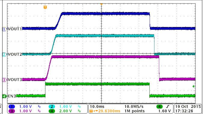
Figure 9-38. Automatic Power Sequencing, MODE = HIGH, EN1 = HIGH, EN2 = LOW
