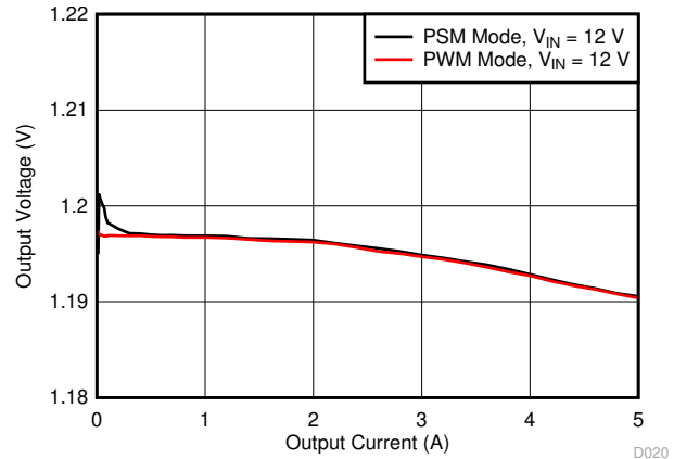
Figure 7-20. Buck1, Load Regulation
