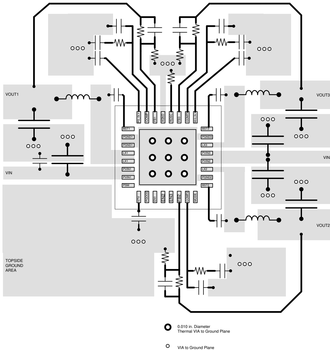
Figure 9-41. PCB Layout
