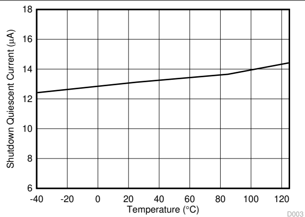
Figure 7-3. Shutdown Quiescent vs Temperature
