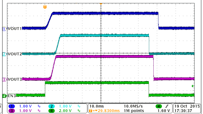
Figure 9-36. Automatic Power Sequencing, MODE = HIGH, EN1 = HIGH, EN2 = HIGH
