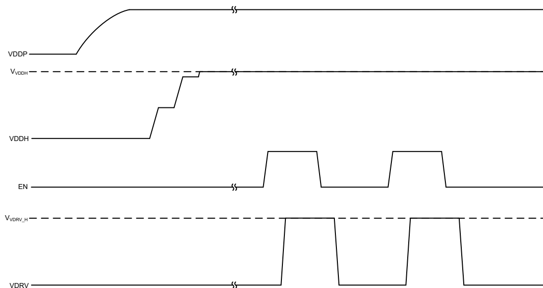
Figure 8-2. Three-Wire Mode with TPSI3050-Q1 (Standard Enable)
