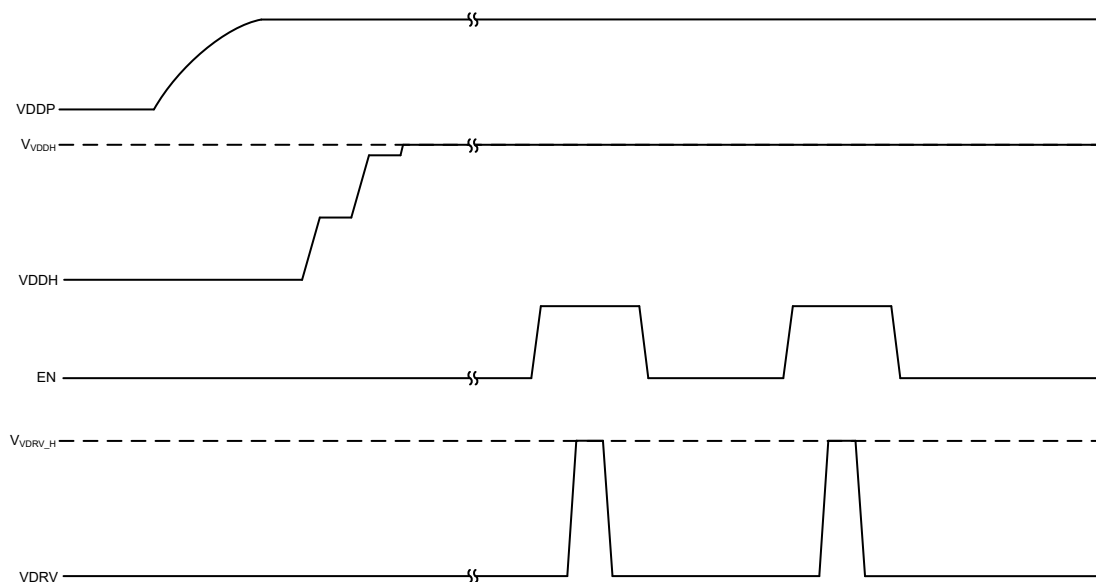
Figure 8-3. Three-Wire Mode with TPSI3050S-Q1 (One-shot Enable)
