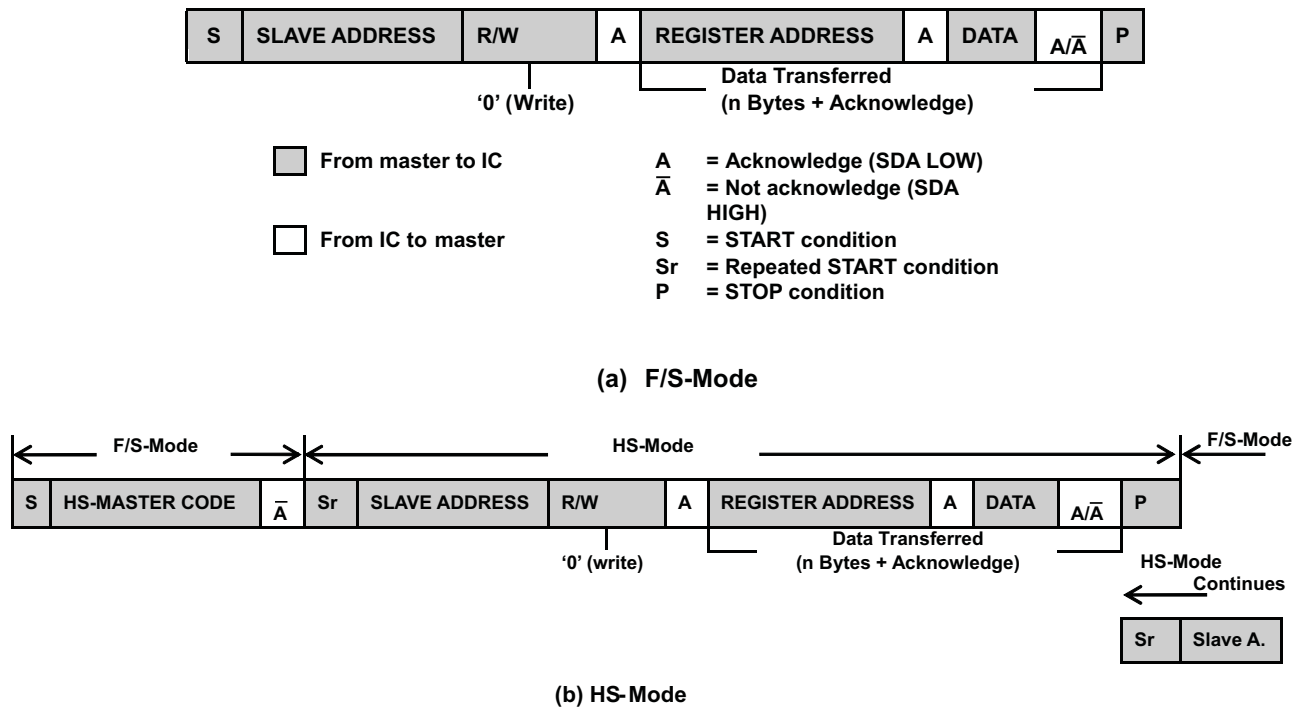
Figure 26. Data Transfer Format In F/S Mode And HS Mode
