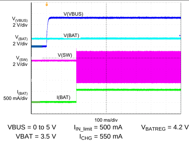
Figure 30. Adapter Insertion (HOST Mode)
