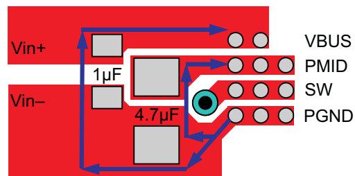
Figure 39. Input Capacitor Position and PCB Layout Example
