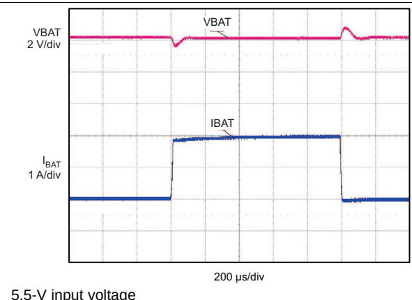
Figure 35. Step Load from 0 to 2 A During Factory Mode
