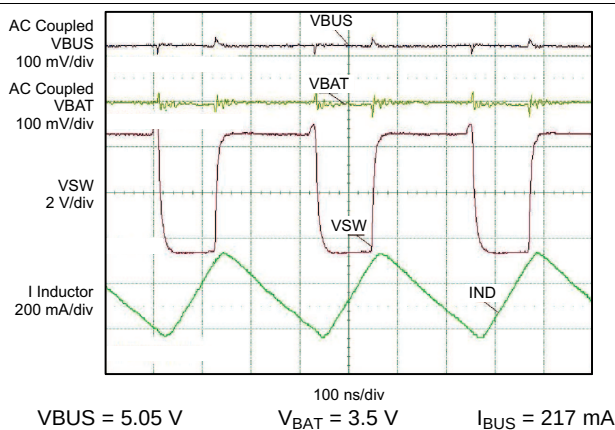
Figure 34. Boost Waveform (PWM Mode)
