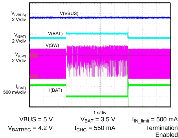
Figure 32. Battery Insertion/Removal Termination Disabled (HOST Mode)
