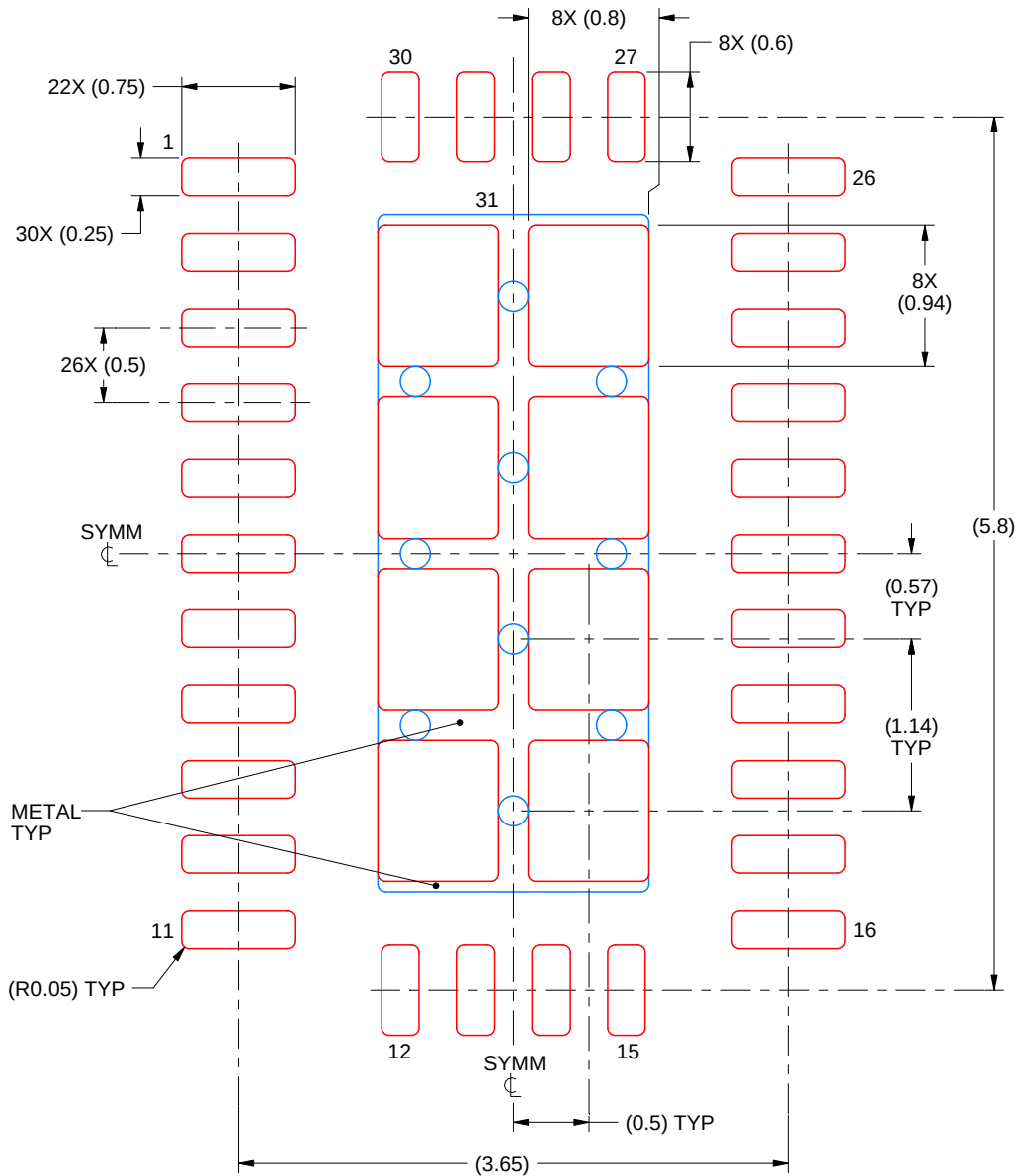
SOLDER PASTE EXAMPLE BASED ON 0.125 mm THICK STENCIL
