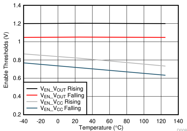
Figure 6-4. Enable Threshold
