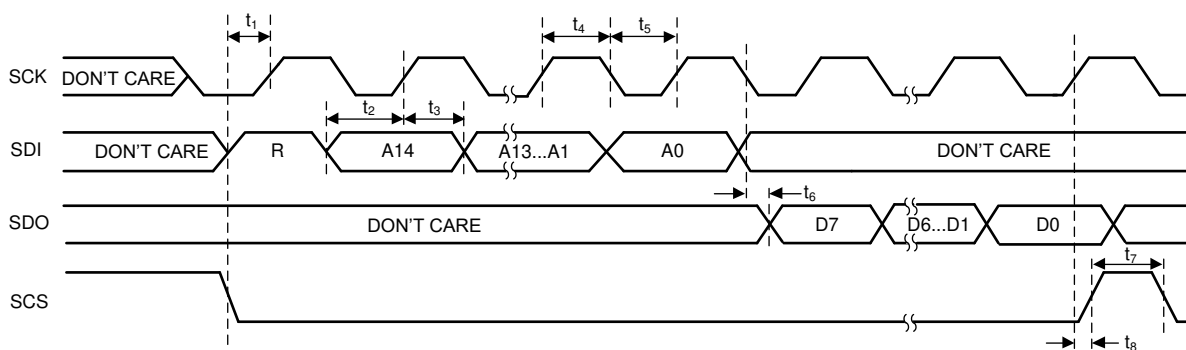
Figure 7-2. SPI 4-Wire Read Timing Diagram
