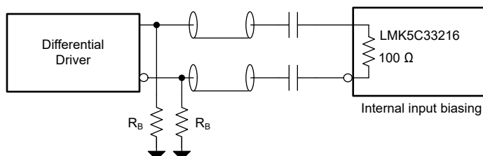
Figure 9-15. AC-Coupled Differential to Reference (INx)
