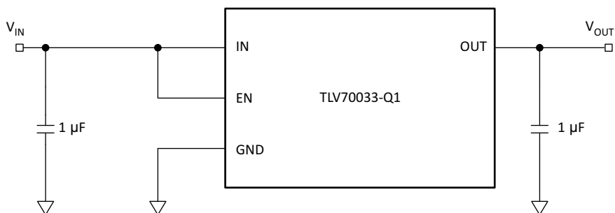
Figure 22. TLV70033-Q1 Typical Application
