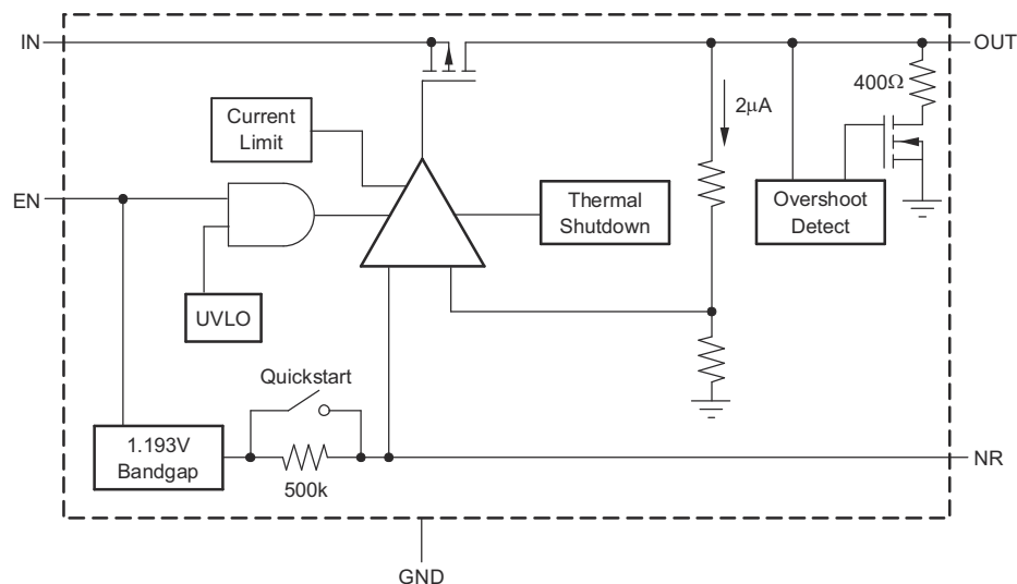
Figure 7-1. Fixed-Voltage Version
