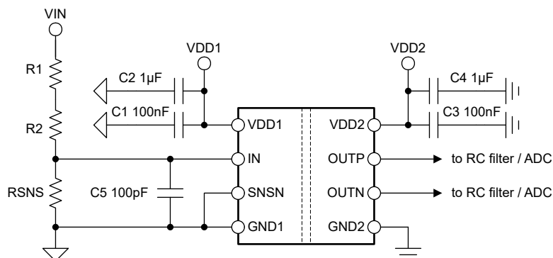
Figure 9-1. Decoupling of the AMC0x30D-Q1
