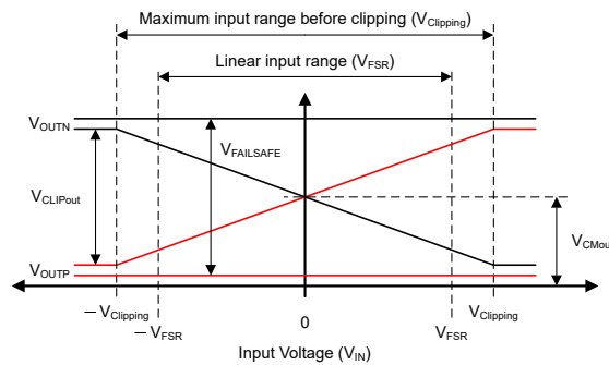
Figure 7-2. Input to Output Transfer Curve of the AMC0x30D-Q1
