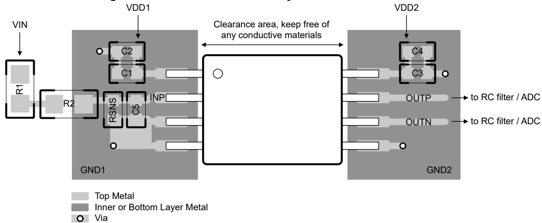
Figure 10-1. Recommended Layout of the AMC0x30D-Q1
