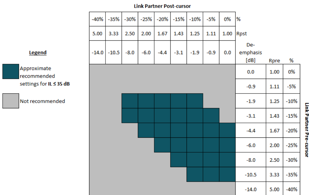
Figure 6-9. Guideline for Link partner FIR Settings When IL \leq 35\text{dB}
