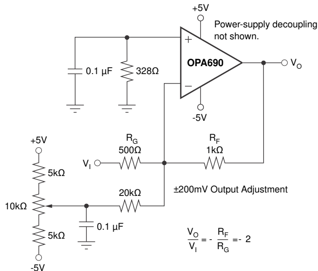
Figure 8-5. DC-Coupled, Inverting Gain of –2 V/V, With Offset Adjustment
