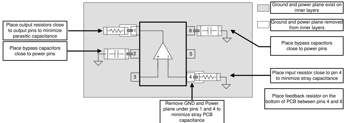
Figure 8-10. OPA690 Layout
