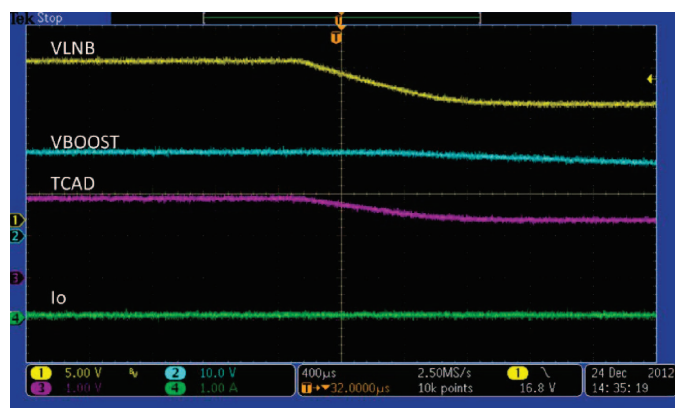
Figure 21. V_{IN} = 12\text{ V} , V_{LNB} = 18.6\text{ V} to 13.4\text{ V} , 0 A, Voltage Transition
