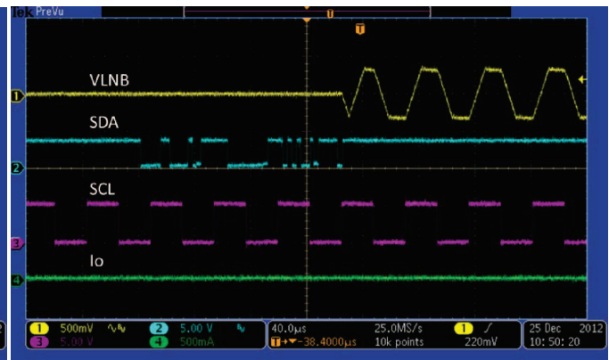
Figure 38. V_{IN} = 12\text{ V} , V_{LNB} = 13.4\text{ V} , No Loading, 22-kHz Tone Delay from I 2 C Gated, EXT M Provides 22 kHz to Output Tone, On
