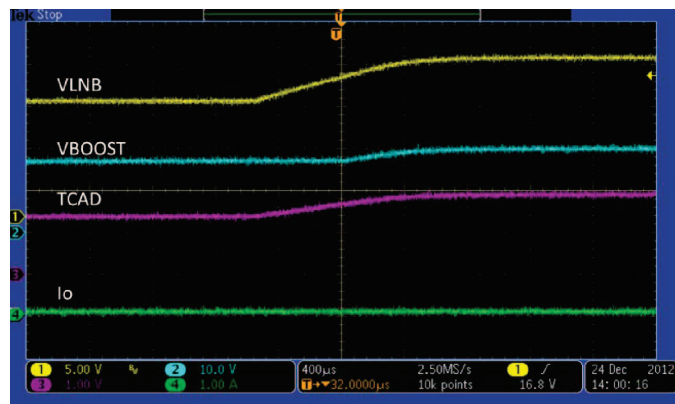
Figure 19. V_{IN} = 12\text{ V} , V_{LNB} = 13.4\text{ V} to 18.6\text{ V} , 0 A, Voltage Transition
