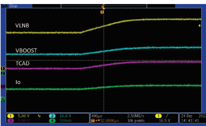
Figure 24. V_{IN} = 5\text{ V} , V_{LNB} = 13.4\text{ V} to 18.6\text{ V} , 0.5 A, Voltage Transition
