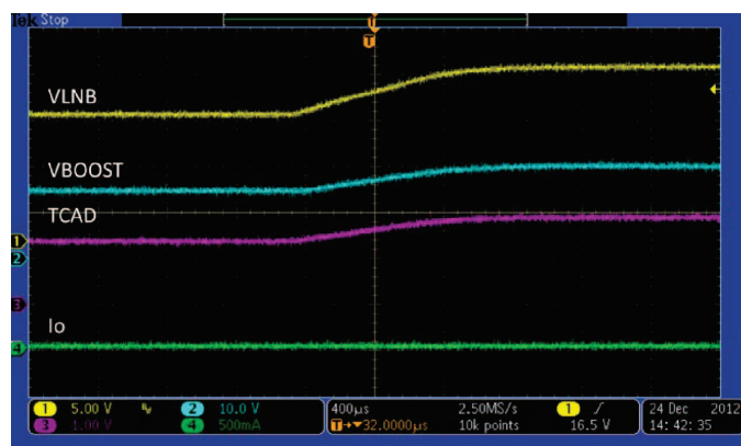
Figure 23. V_{IN} = 5\text{ V} , V_{LNB} = 13.4\text{ V} to 18.6\text{ V} , 0 A, Voltage Transition
