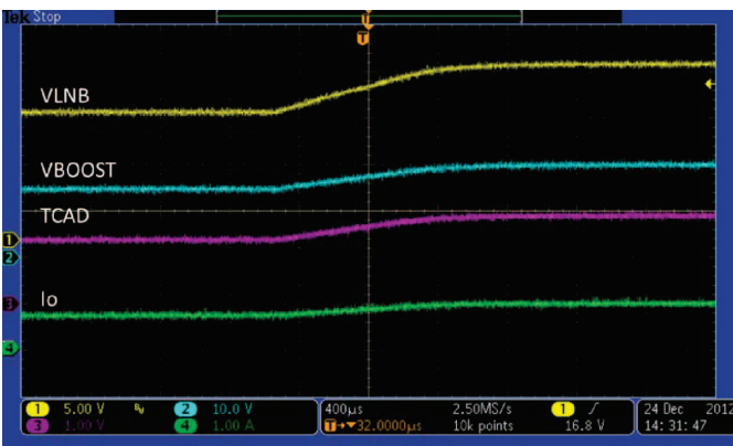
Figure 20. V_{IN} = 12\text{ V} , V_{LNB} = 13.4\text{ V} to 18.6\text{ V} , 1 A, Voltage Transition
