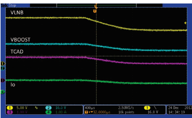
Figure 22. V_{IN} = 12\text{ V} , V_{LNB} = 18.6\text{ V} to 13.4\text{ V} , 1 A, Voltage Transition
