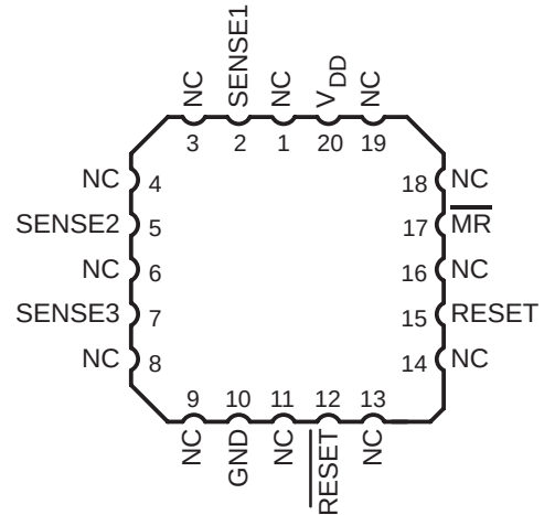
FK PACKAGE (TOP VIEW)
