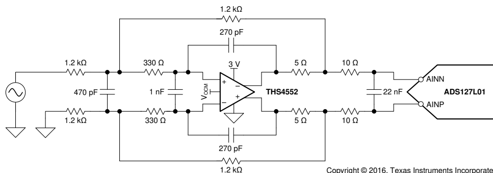
Simplified Schematic: Gain of 1-V/V, Single-Ended Input to Differential Output, 500-kHz, Multiple Feedback Filter Interface to the ADS127L01 (1 of 2 Channels)
