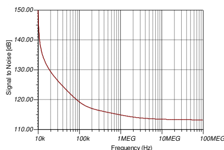
Figure 9-16. Signal-to-Noise Ratio Plot
