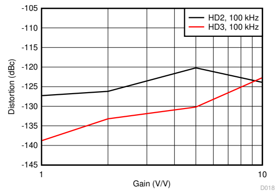
Figure 6-18. Harmonic Distortion vs Gain
