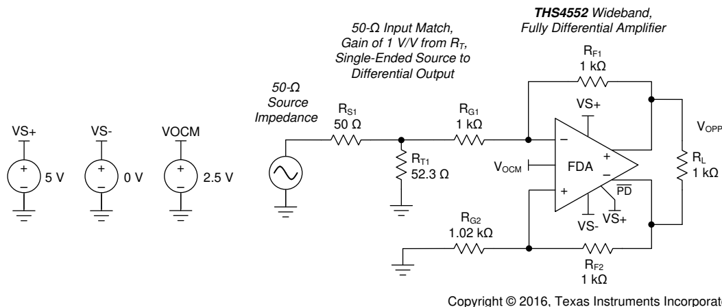
Figure 8-9. DC-Coupled Gain of 1 with R_F = 1 \text{ k}\Omega and Single-to-Differential Matched Input 50 Ω Impedance
