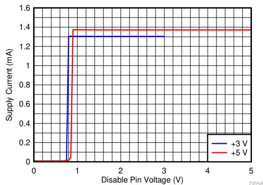
Figure 6-56. Supply Current vs PD Voltage
