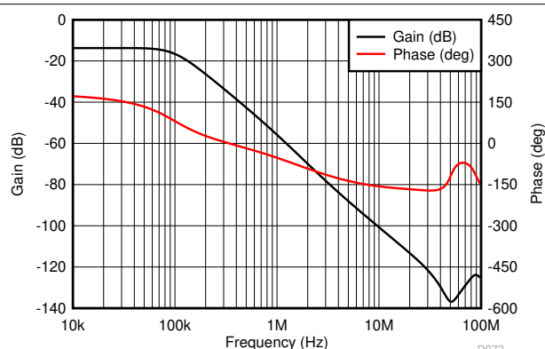
Figure 9-15. Gain and Phase Plot for a 100 kHz Butterworth Filter
