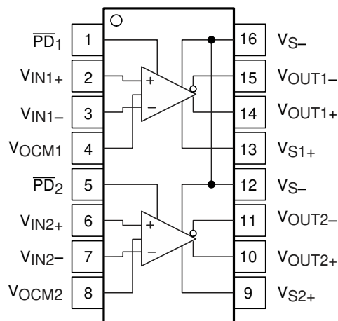
Figure 5-2. PW Package 16-Pin VSSOP Top View
