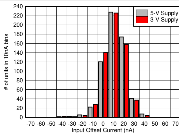
600 units at each supply voltage Figure 6-44. Input Offset Current Distribution
