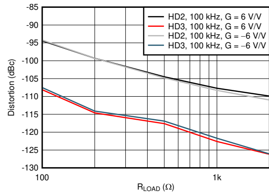
Figure 6-14. Harmonic Distortion vs R_{LOAD}
