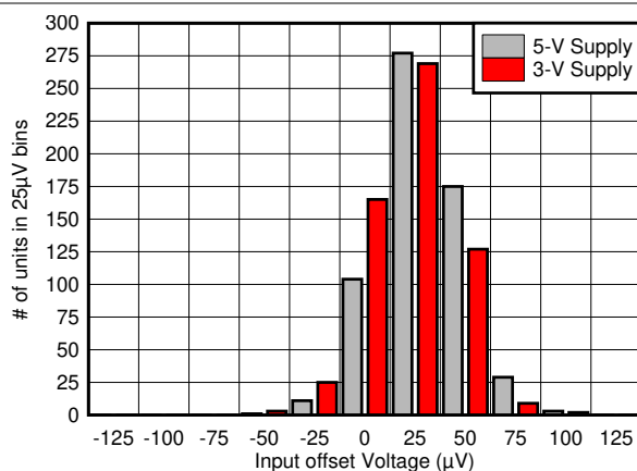
600 units at each supply voltage Figure 6-43. Input Offset Voltage Distribution
