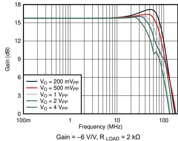
Figure 6-4. Inverting Large-Signal Bandwidth vs V_{OPP}
