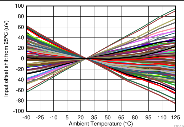
51 units at 5-V and 3-V supply Figure 6-45. Input Offset Voltage vs Temperature
