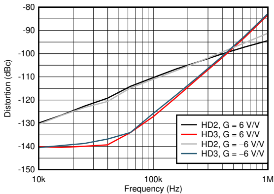
Figure 6-13. Harmonic Distortion vs Frequency
