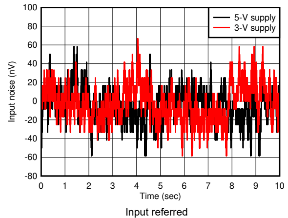
Figure 6-40. Low-Frequency Voltage Noise
