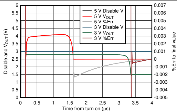
Figure 6-52. Turn-Off Time to Sinusoidal Input
