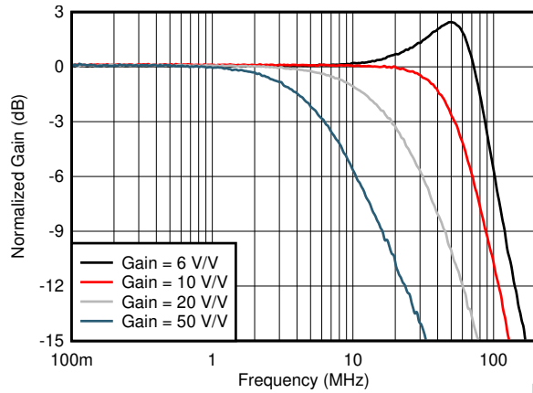
Figure 6-1. Noninverting Small-Signal Frequency Response vs Gain
