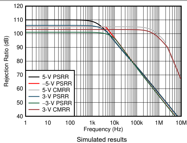
Figure 6-41. PSRR and CMRR
