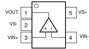
Figure 5-2. DCK Package, 5-Pin SC70 (Top View)
