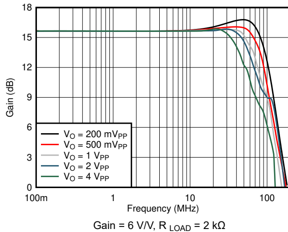
Figure 6-3. Noninverting Large-Signal Bandwidth vs V_{OPP}
