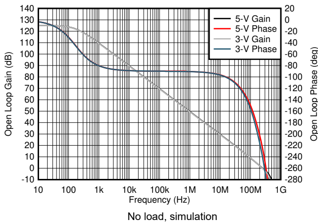
Figure 6-37. Open-Loop Gain and Phase
