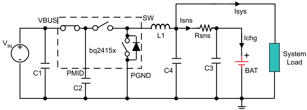
Figure 35. System Load Before Sensing Resistor
