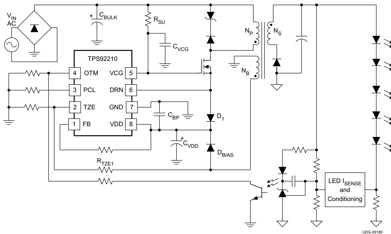
Figure 17. Typical Application
