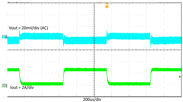
Figure 7-21. TPS563206 Load Transient With 0.3A to 2.7A
