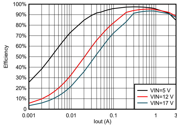
Figure 5-15. TPS563206 Efficiency at 3.3 Vout With 4.7uH Inductor
