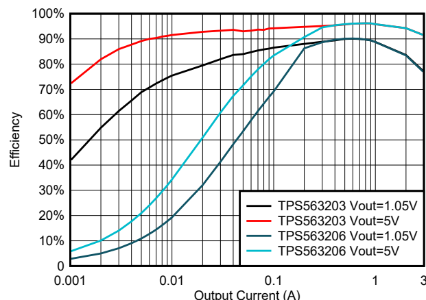
TPS563203 and TPS563206 Efficiency
