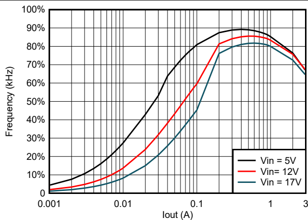
Figure 5-11. TPS563206 Efficiency at 0.6 Vout With 1.5uH Inductor
