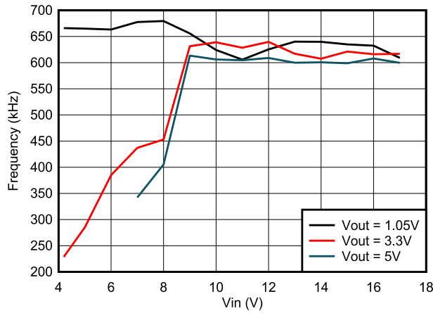
Figure 5-7. Frequency vs Input Voltage at 3A Loading
