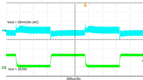
Figure 7-20. TPS563203 Load Transient With 0.3A to 2.7A
