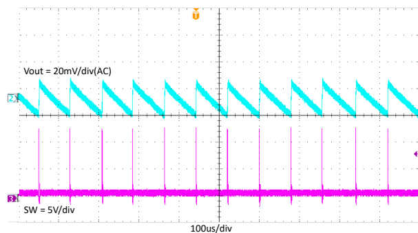
Figure 7-8. TPS563203 Output Voltage Ripple With 0.1A Loading
