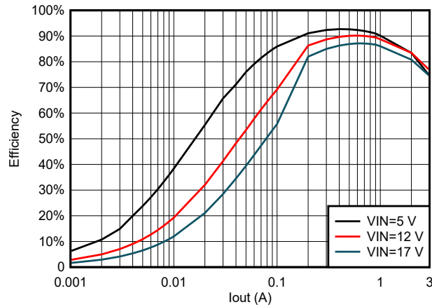
Figure 5-13. TPS563206 Efficiency at 1.05 Vout With 2.2uH Inductor
