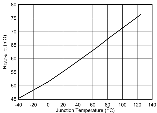
Figure 5-5. Low-Side R_{dson}
