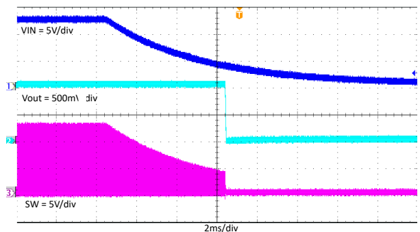
Figure 7-19. TPS563206 Power off With 3A Loading
