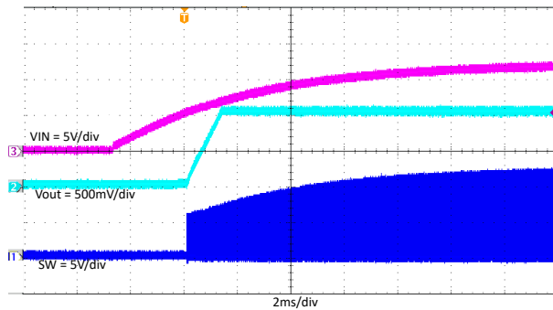
Figure 7-16. TPS563203 Power on With 3A Loading
