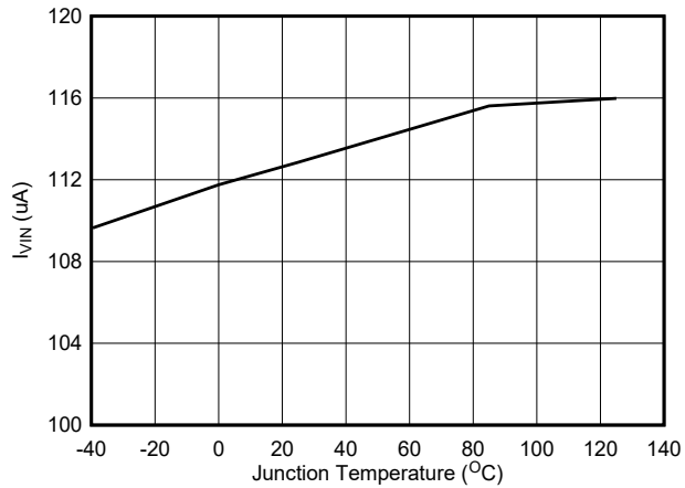
Figure 5-1. TPS563203 Quiescent Current
