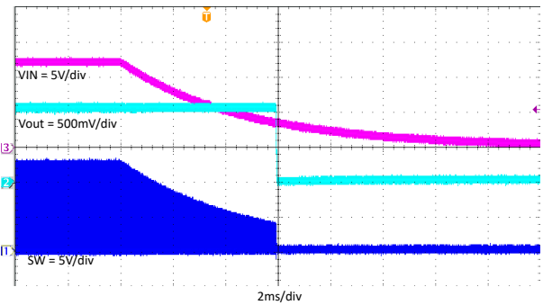
Figure 7-17. TPS563203 Power off With 3A Loading
