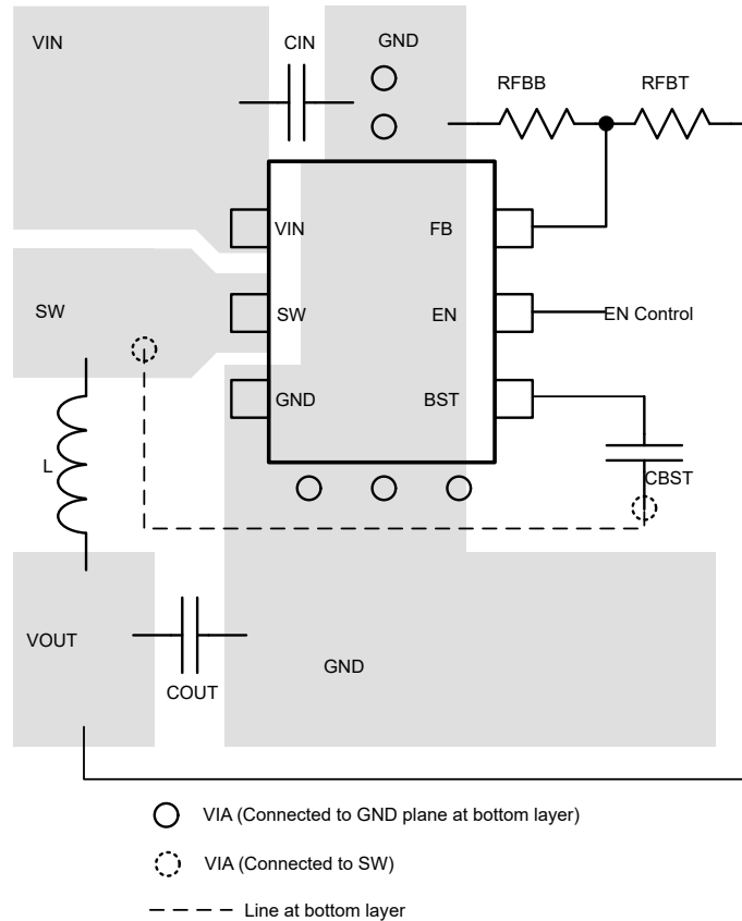
Figure 7-22. TPS563203 Layout
