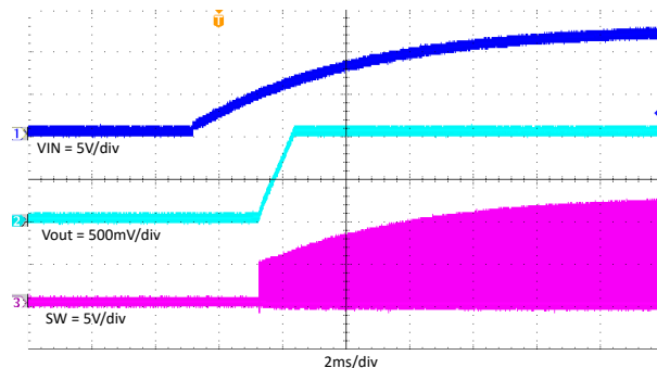
Figure 7-18. TPS563206 Power on With 3A Loading
