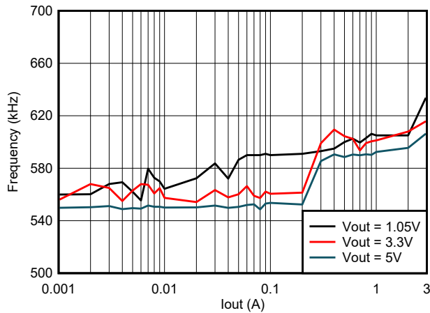
Figure 5-9. TPS563206 Frequency vs Loading
