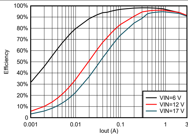
Figure 5-17. TPS563206 Efficiency at 5 Vout With 4.7uH Inductor
