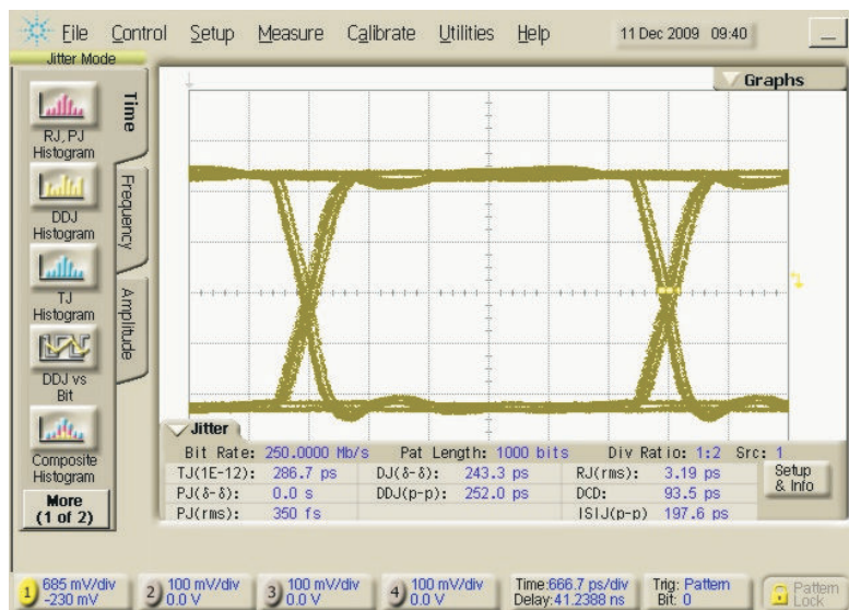
Figure 5-11. Output ( V_{CC} = 3.3V , V_{ID} = 400mV ) 250Mbps 2^{15} -1PRBS, Receiver Type 1
