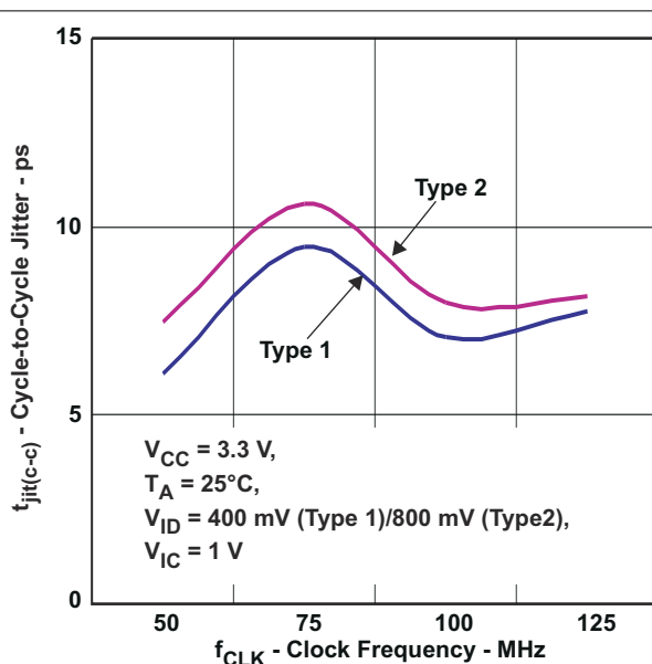
Figure 5-10. Added Receiver Cycle-to-Cycle Jitter vs Clock Frequency
